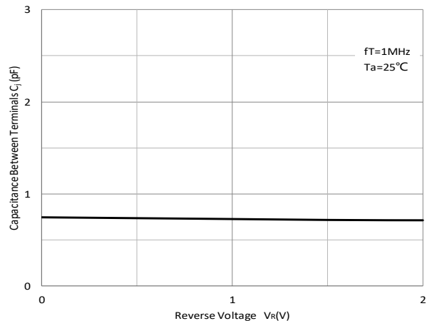
Fig 2: Capacitance Capability
