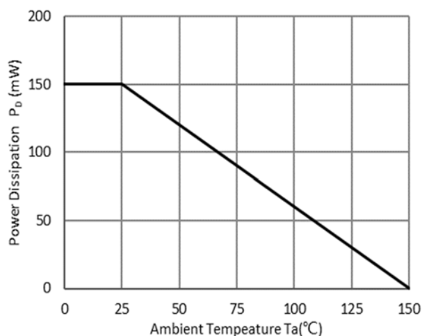
Fig 6: P_D-Ta Curve
