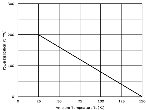
Fig 5: PD-Ta Curve
