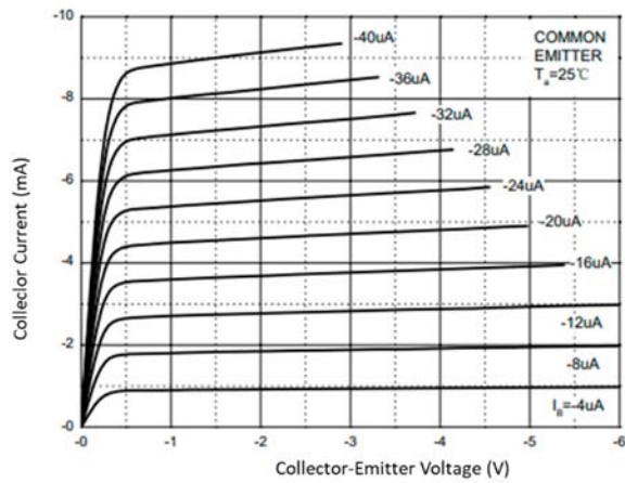
Fig 1: Static Characteristics
