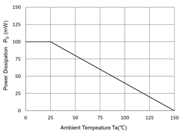
Fig 6: P_D-Ta Curve
