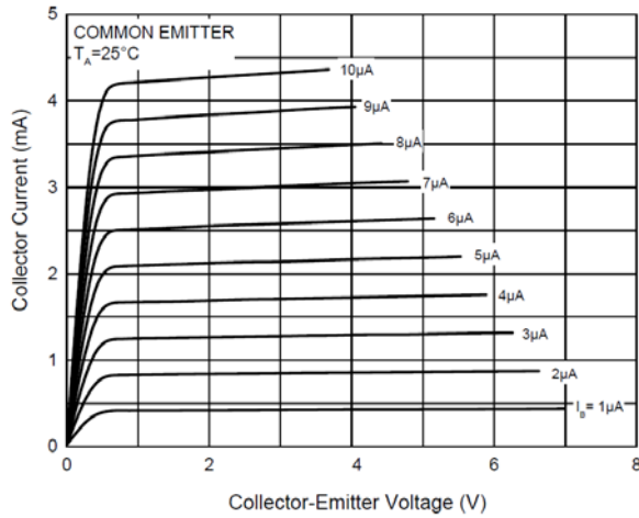
Fig 1: Static Characteristics
