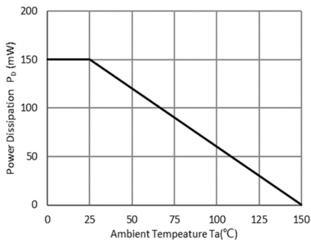
Fig 5: P_D-Ta Curve
