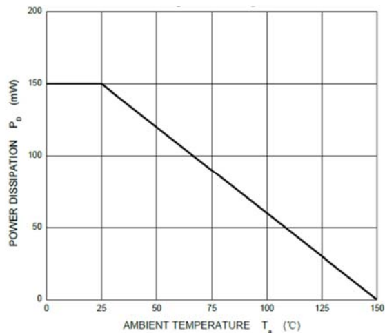
Fig 6: P_D-Ta Curve
