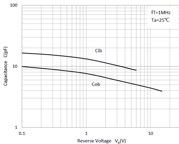
Fig 6: Cob/Cib- V_{CB}/V_{EB}
