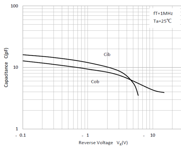
Fig 6: C_{ob}/C_{ib}-V_{CB}/V_{EB}
