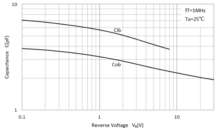
C_{ob}/C_{ib}-V_{CB}/V_{EB}
