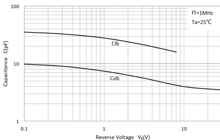
C_{ob}/C_{ib}-V_{CB}/V_{EB}
