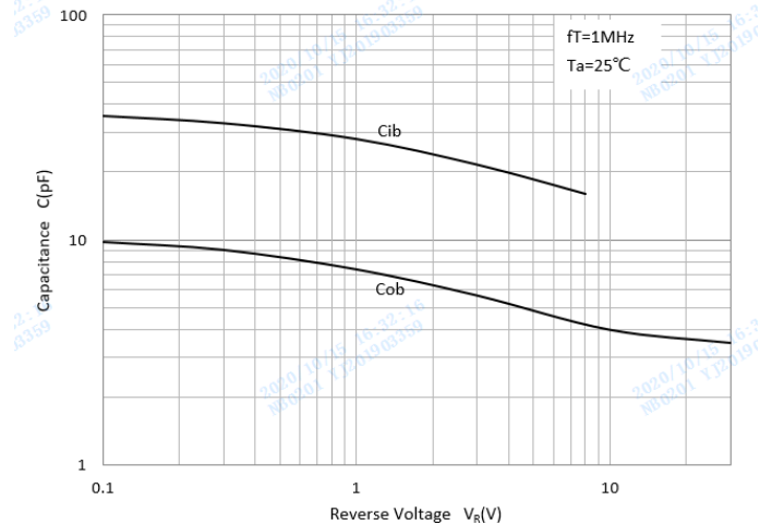
C_{ob}/C_{ib}-V_{CB}/V_{EB}
