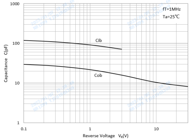
C_{ob}/C_{ib}-V_{CB}/V_{EB}
