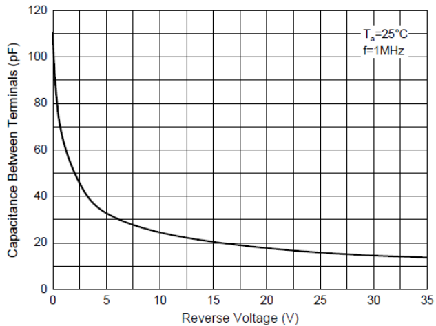
Fig. 3 - Capacitance Characteristics
