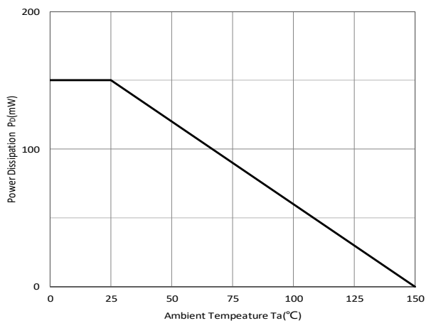
Fig 5: P<sub>D</sub>-T<sub>a</sub> Curve
